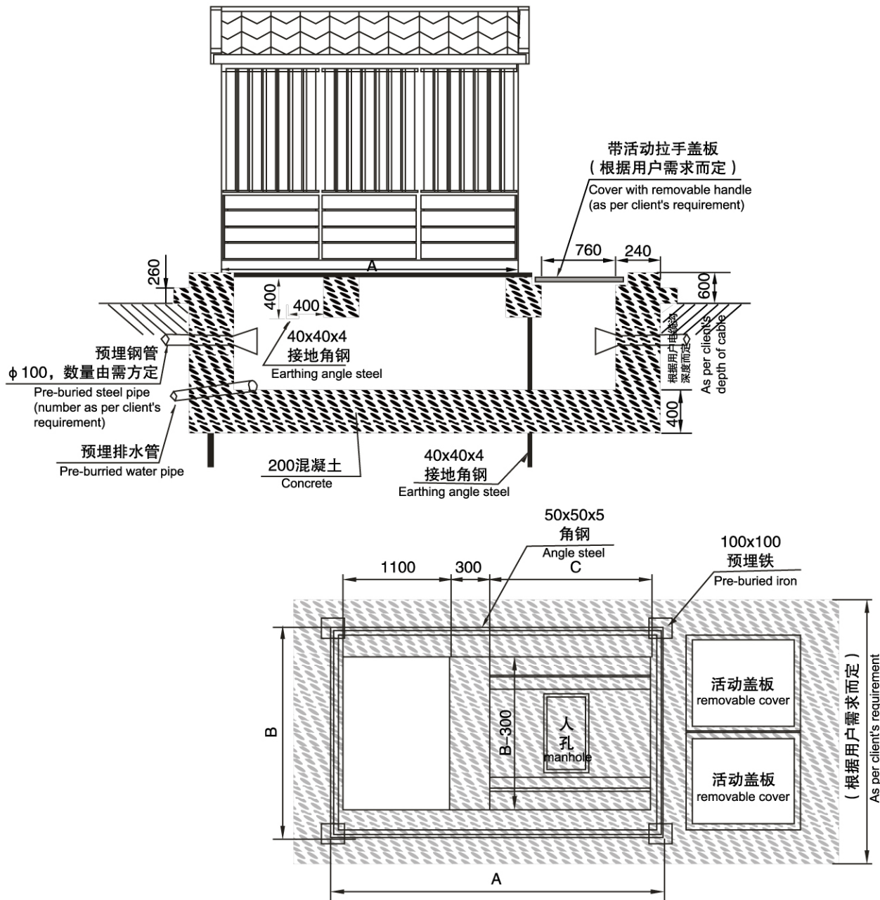
MK1、MK2、MK3 Enclosure Foundation Diagram
