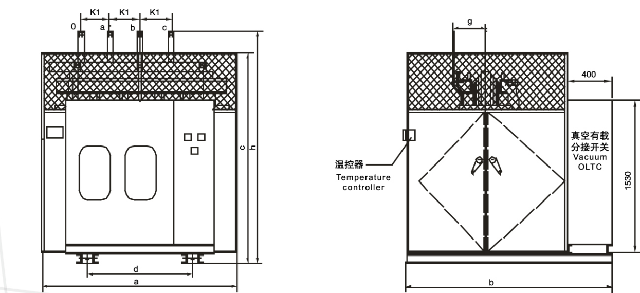
SC(B)Z9有载调压干式配电变压器带IP20保护外壳外形图 Outline diagram of SC (B) Z9 Dry-type distribution transformer with IP20 protection enclosure
